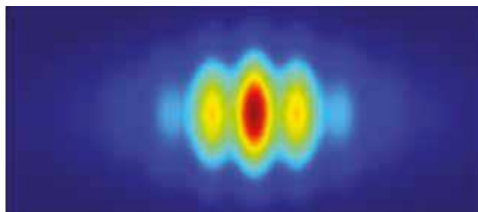
FIGURE 3 (below). Expected atomic interference pattern.
